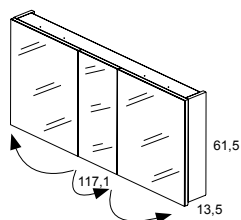
Camerino 120 3P BINOVA F-13,5 / BINOVA cupboard 120 3D D-13,5
